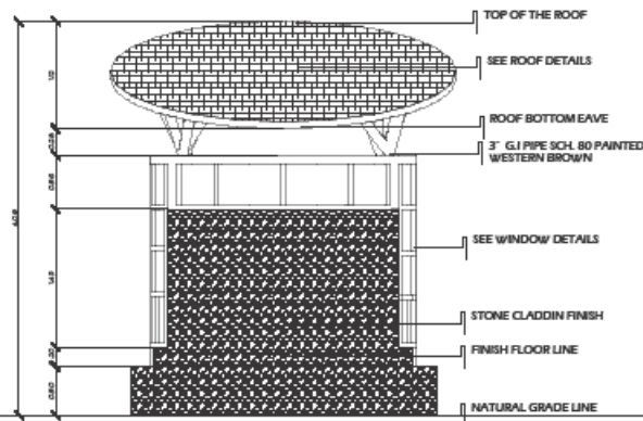
4 REAR ELEVATION A/S SCALE: 150MTRS.
