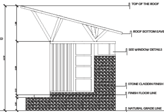
5 RIGHT SIDE ELEVATION A/S SCALE: 150MTRS.
