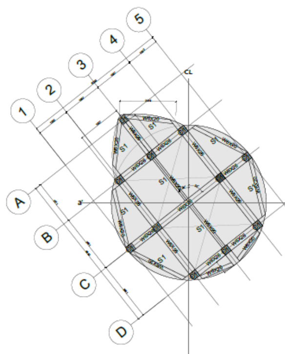
1 DECK 1 BEAM AND COLUMN PLAN REV 12/22
