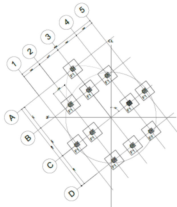
2 DECK 1 FOUNDATION PLAN REV 12/22
