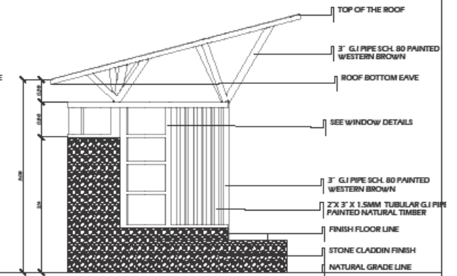
6 LEFT SIDE ELEVATION A/S SCALE: 150MTRS.
