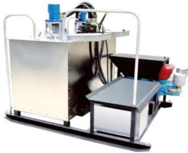
Thermoplastic Paint Preheater (Kneader machine) (Single cylinder; diesel engine; paint capacity: 1500kg; heating method: LPG; truck mounted, with complete accessory, w/ 1 year warranty)
