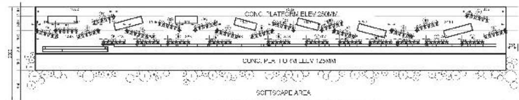
3 TUBULAR SCREEN SETTING LAYOUT 1:200
