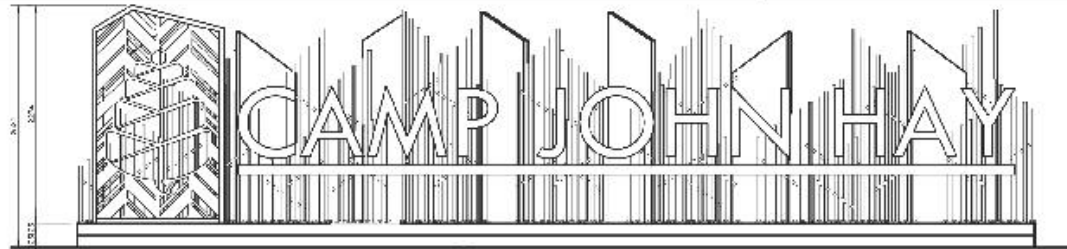
4 FRONT ELEVATION 1:200
