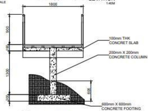
4 BOARDWALK SECTION SCALE 1:40M
