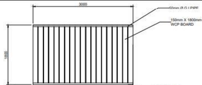
2 BOARDWALK TYPICAL PLAN SCALE 1:40M
