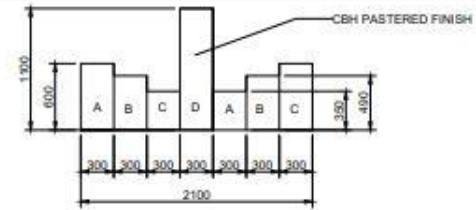
2 STEPPED WALKWAY TYPICAL PLAN SCALE: A10 1:40M
