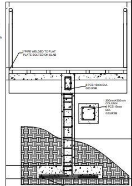
5 BOARDWALK SECTION 2 SCALE 1:40M
