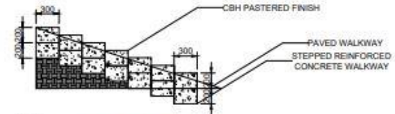
3 STEPPED WALKWAY SECTION SCALE: A10 1:40M
