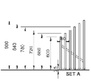
3 SCHEDULE OF COMPONENTS (WALL AND SCREENS) 1/200
