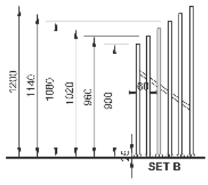
3 SCHEDULE OF COMPONENTS (WALL AND SCREENS) 1/200
