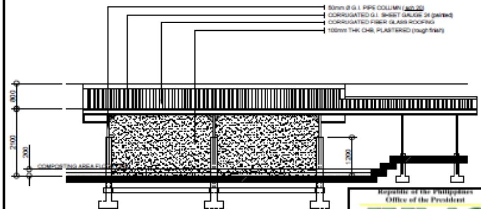
REAR ELEVATION SCALE 1:80m
