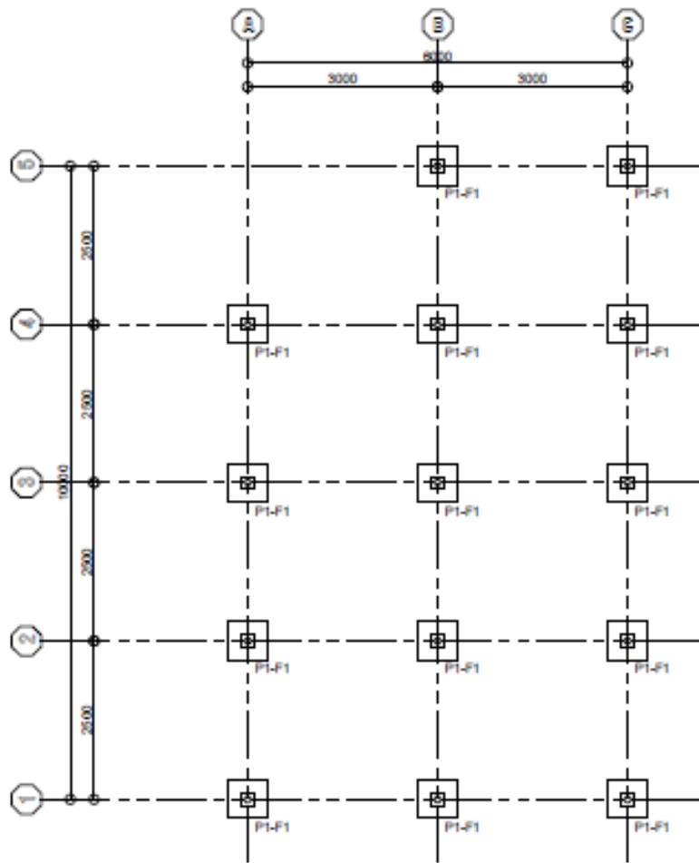
FOUNDATION PLAN SCALE 1:75m
