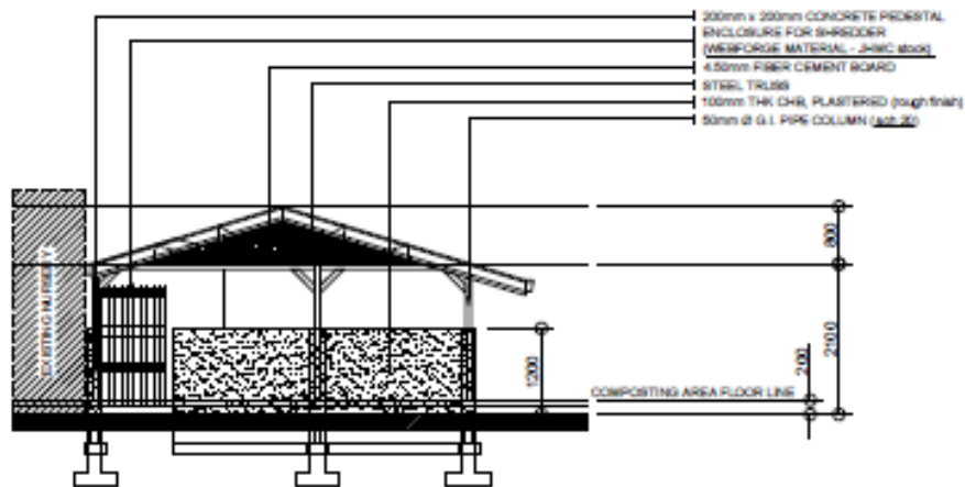
LEFT SIDE ELEVATION SCALE 1:80m
