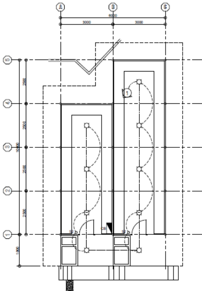
LIGHTING LAYOUT SCALE 1:80m
