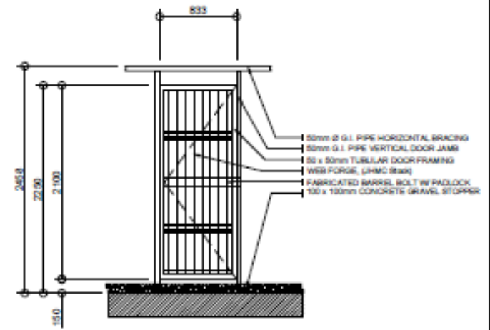
STEEL DOOR DETAIL SCALE 1:40m
