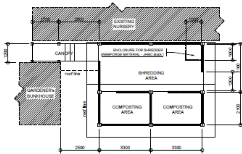
FLOOR PLAN SCALE 1:100m
