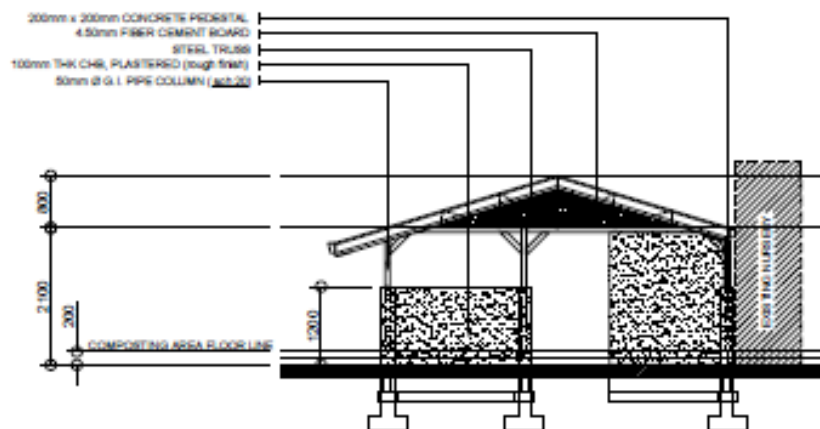
RIGHT SIDE ELEVATION SCALE 1:80m
