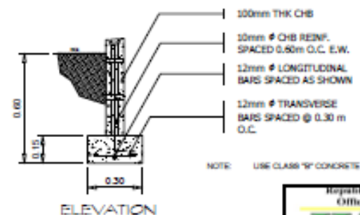
WALL FOOTING DETAIL SCALE 1:20m
