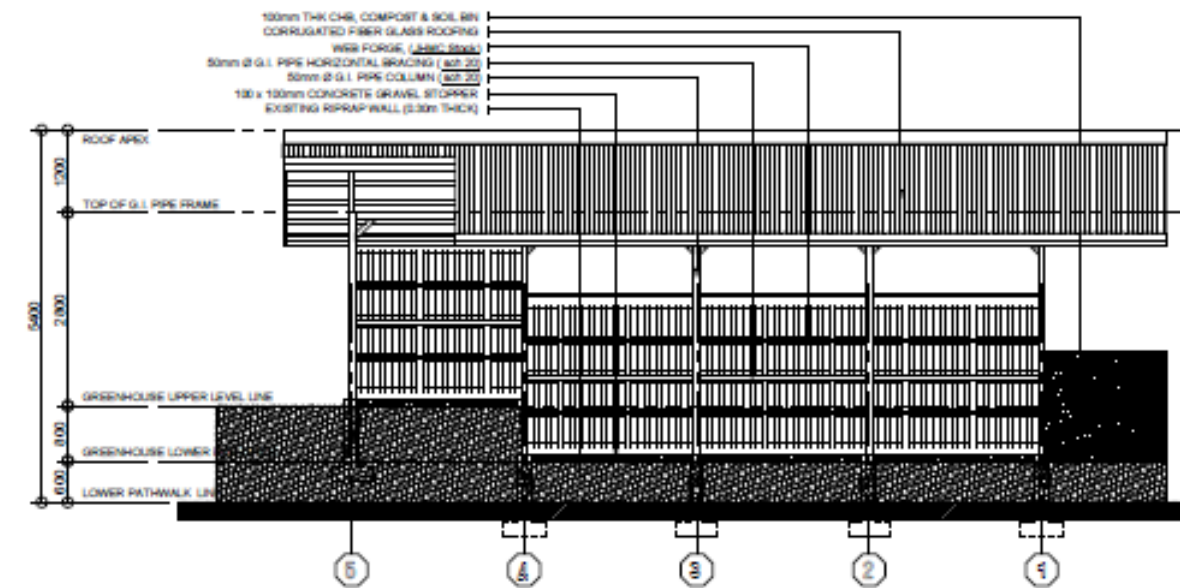
LEFT SIDE ELEVATION SCALE 1:75m
