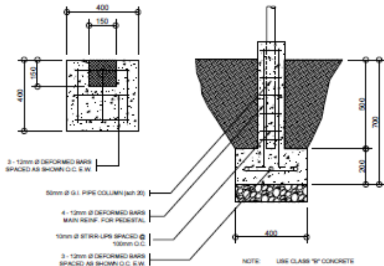
PEDESTAL - FOOTING (P3-F3) DETAIL SCALE 1:15m
