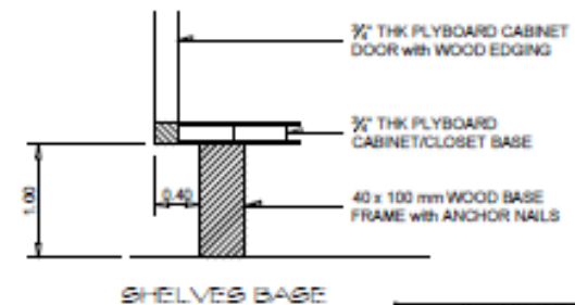
CABINET DETAILS SCALE 1:5m
