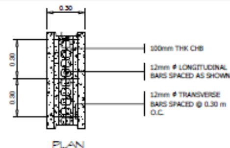
PEDESTAL - FOOTING (P2-F2) DETAIL SCALE 1:20m
