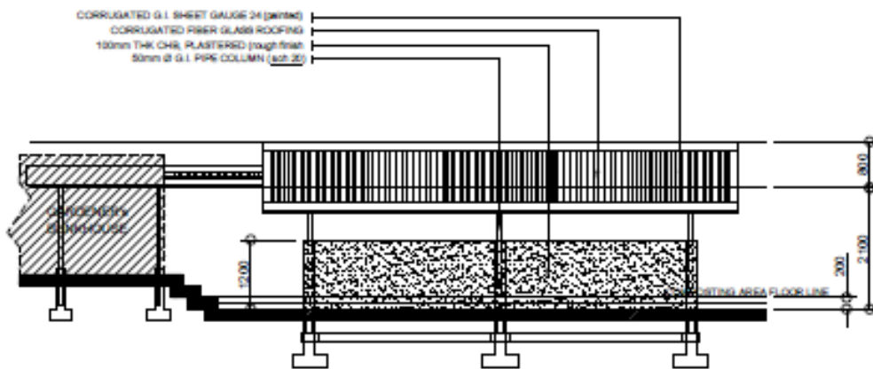
FRONT ELEVATION SCALE 1:80m
