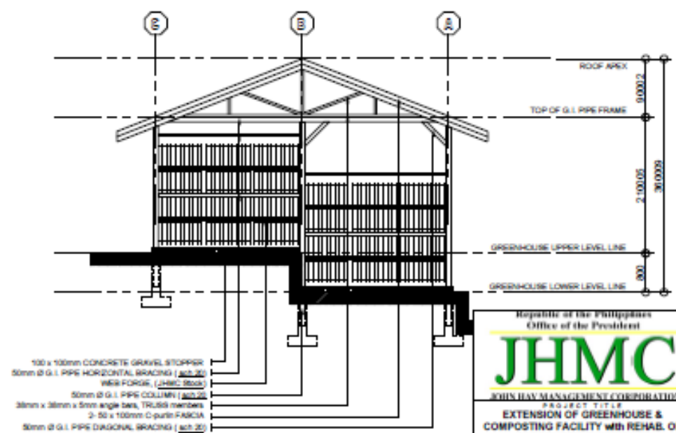
REAR ELEVATION SCALE 1:75m
