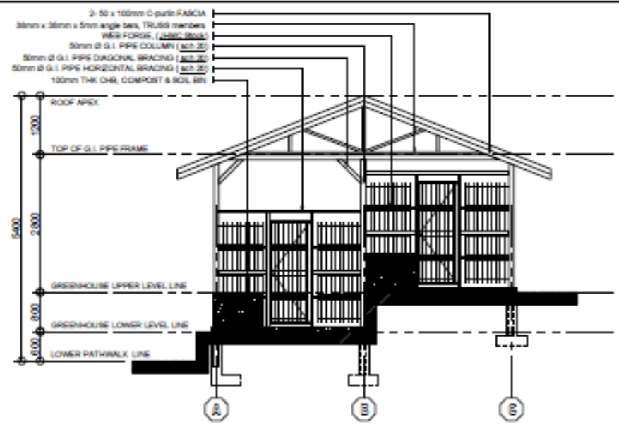
FRONT ELEVATION SCALE 1:75m
