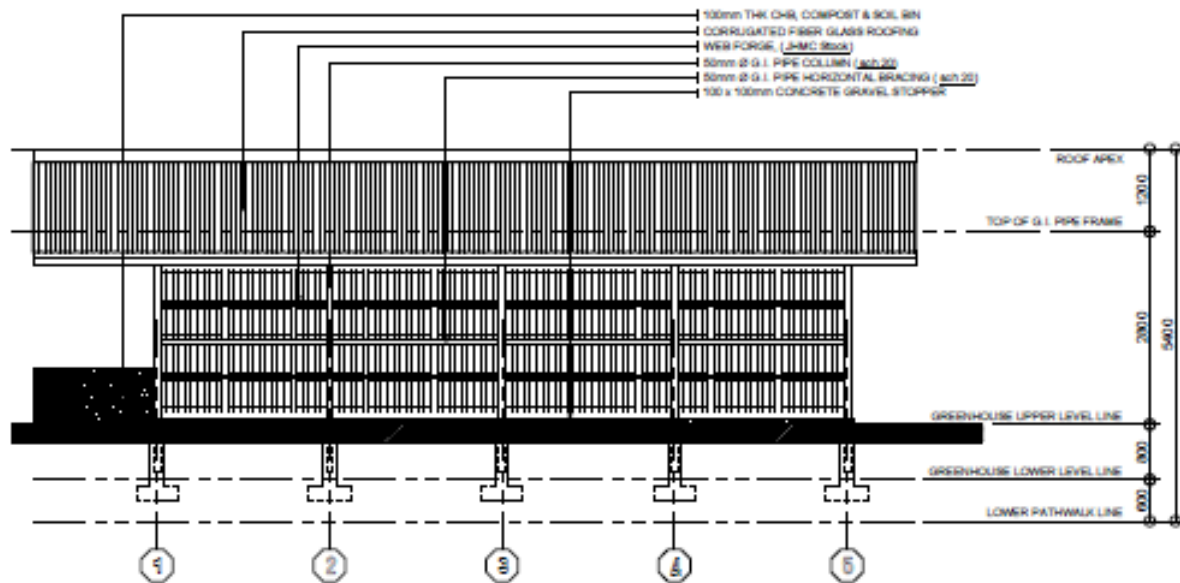
RIGHT SIDE ELEVATION SCALE 1:75m
