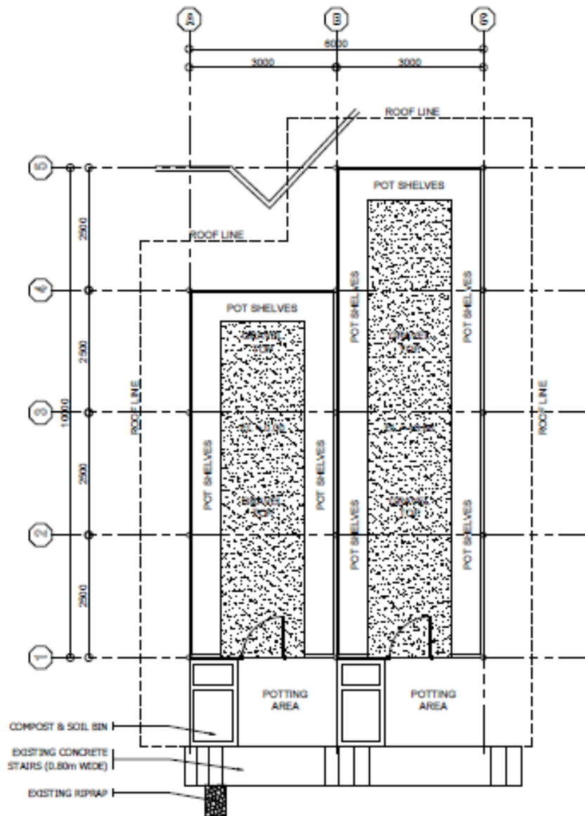
FLOOR PLAN SCALE 1:75m
