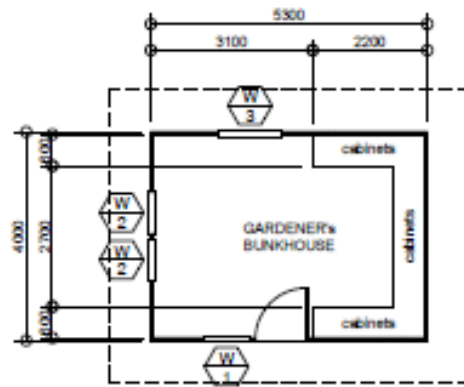
FLOOR PLAN SCALE 1:100m
