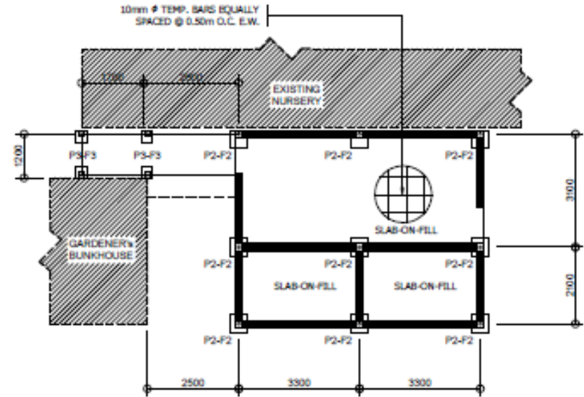
FOUNDATION PLAN SCALE 1:100m
