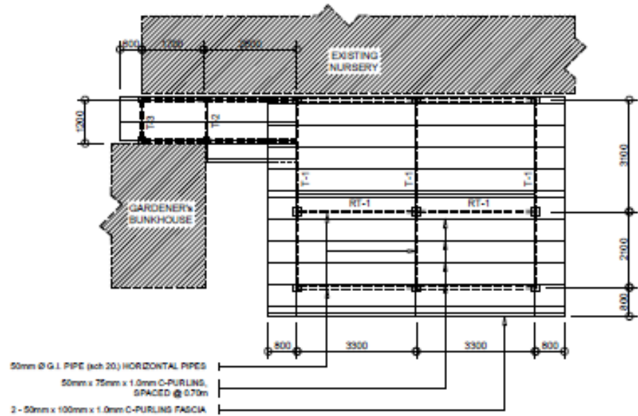
ROOF FRAMING PLAN SCALE 1:100m
