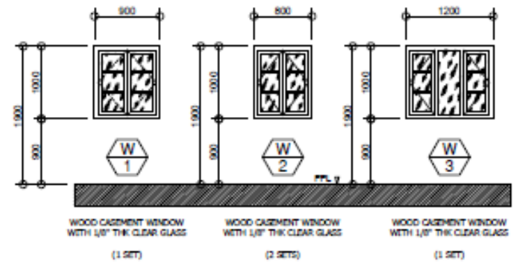
WINDOW DETAIL & SCHEDULE SCALE 1:50m
