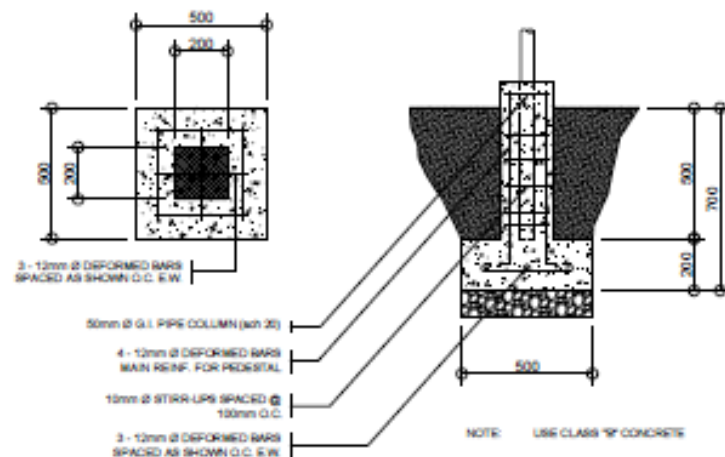
PEDESTAL - FOOTING (P2-F2) DETAIL SCALE 1:20m
