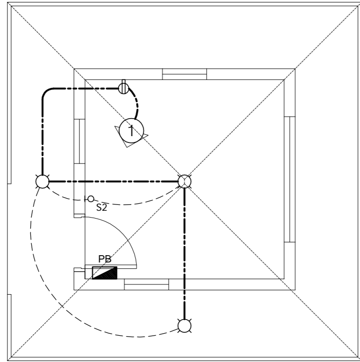
TYPICAL ELECTRICAL LAYOUT SCALE 1:50m
